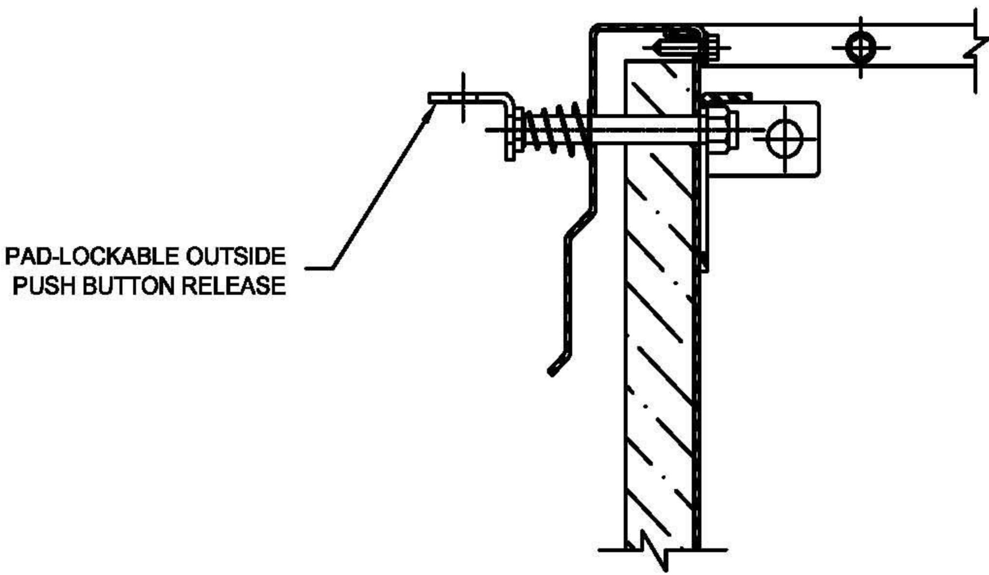
VIEW "A"
